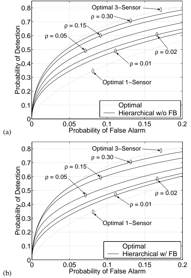
Fig. 2. ROCs for 3-sensor example (a) without feedback and (b) with feedback. Plots show the optimal 1 and 3-sensor ROC and the hierarchical ROC for \rho = 0.30, 0.15, 0.05, 0.02, and 0.01 .
