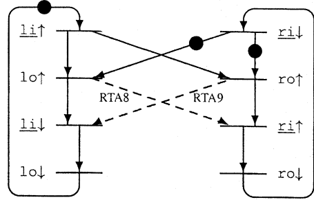
Fig. 9. FIFO specification Petri-net, with RT assumptions RTA8 and RTA9 represented as dashed arcs.
