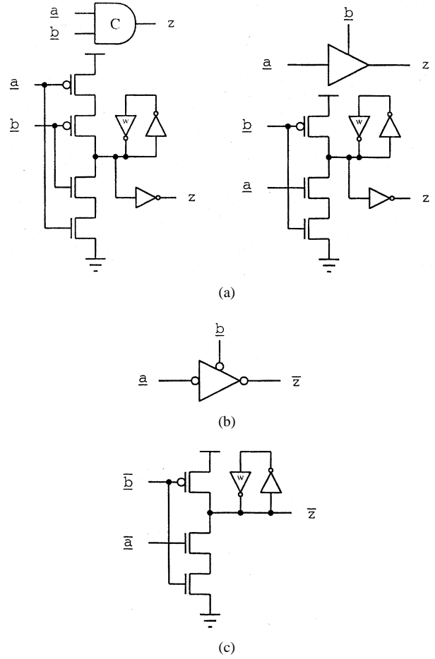
Fig. 2. Generalized C-elements: (a) GC, (b) GC-RT for \underline{a} \downarrow \prec \underline{b} \downarrow , and (c) for \underline{a} \uparrow \prec \underline{b} \uparrow .
