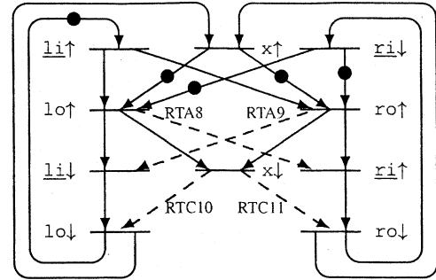
Fig. 11. Petri-net for circuit of Fig. 10 and constraints RTC10–RTC11.
