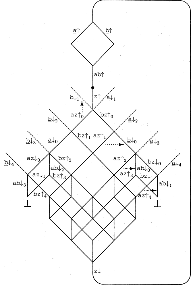
Fig. 5. Relative timed burst-mode SC state graph.
