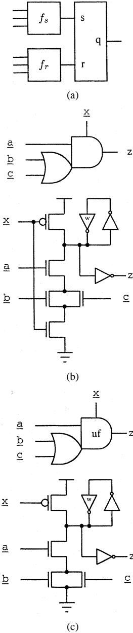
Fig. 1. (a) Set-reset flop and functions. (b) Footed domino gate (symbol and circuit) implementing a set-reset flop with f_r = \bar{x} , f_s = x \times a \times (\bar{b} + \bar{c}) . (c) Unfooted domino gate implementing f_r = \bar{x} , f_s = a \times (\bar{b} + \bar{c}) .
