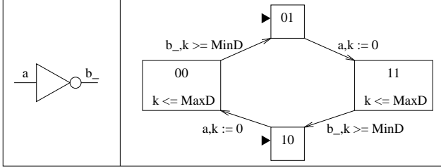
Figure 1. Simple Inverter Logic Symbol and TSA
