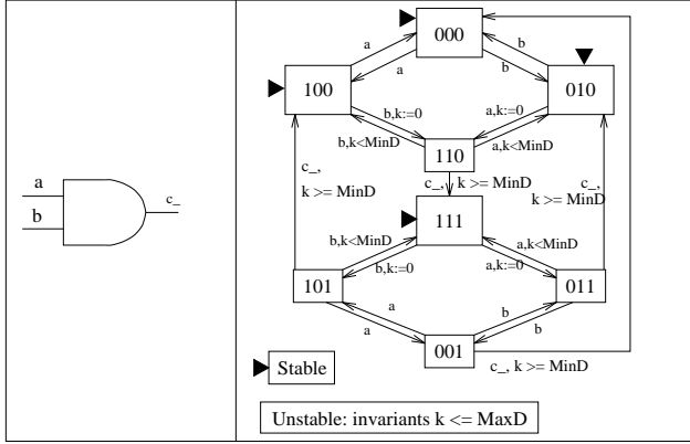
Figure 2. Two-Input And-Gate
