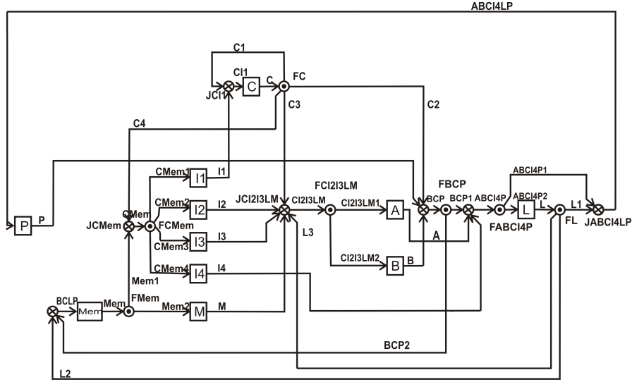
Fig. 21. CNG-optimized control network of the elastic clocked MiniMIPS [11].
