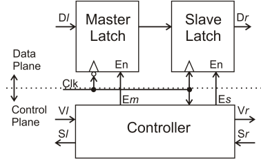
Fig. 1. An EB implementation.
