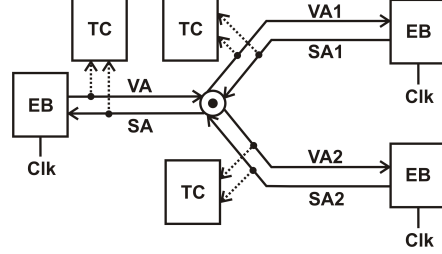
Fig. 6. Lazy fork verification setup.
