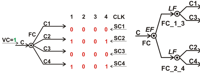
Fig. 22. Stall patterns at the branches of FC in the presence of bubbles.
