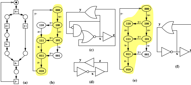
Fig. 2: (a) STG for the xyz example, (b,e) SGs with timing domains, (c,d,e) Circuits.
