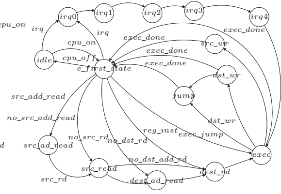
Fig. 3. Execute State Machine for MSP430
