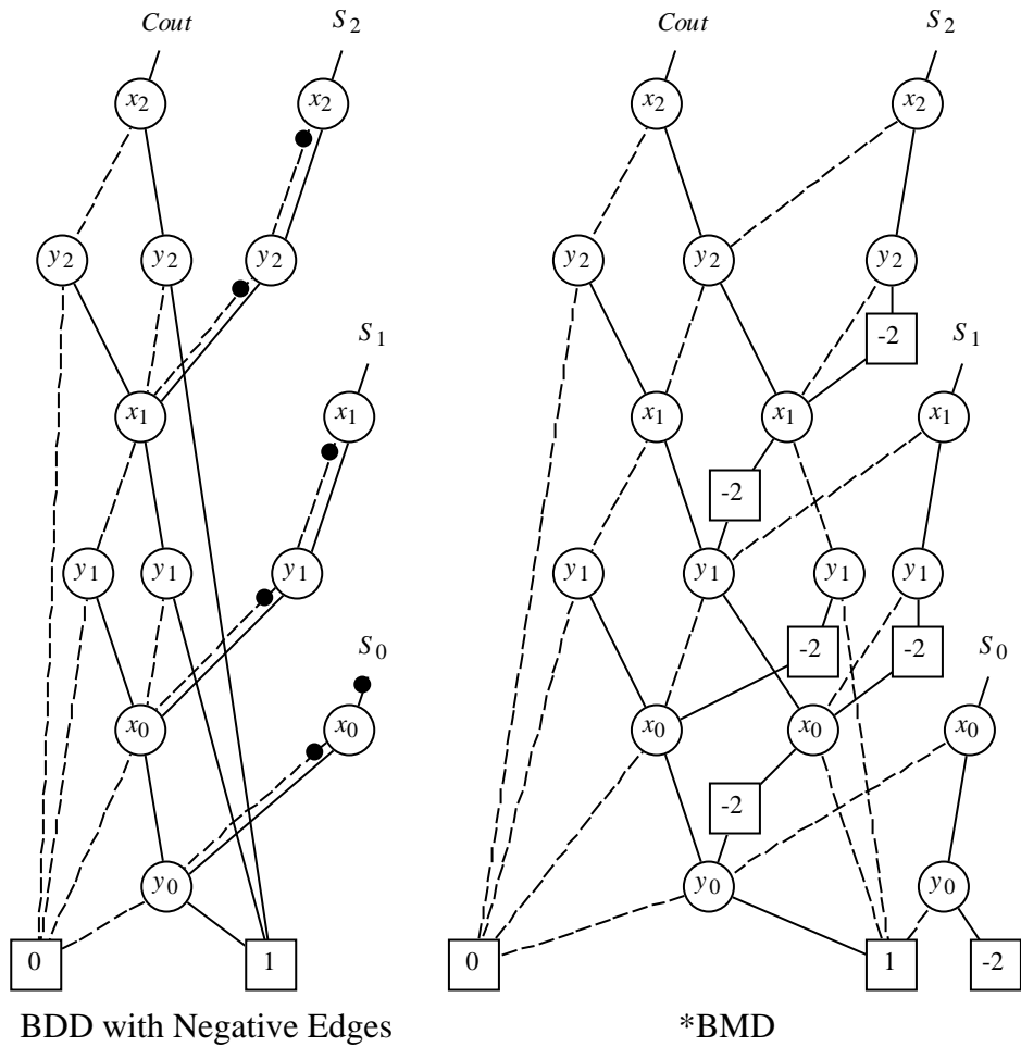
Figure 9: Bit-Level Representations of Addition Functions. Each graph represents all four outputs of a 3-bit adder.
