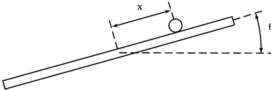
Figure 8.31: Ball and Beam System
