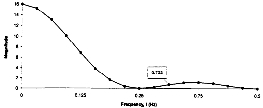
3. Magnitude spectrum X_1(f) for the signal x_1(t) , plotted at the frequencies f = k/32 on 0 \leq f \leq 1/2 . Since the signal is real and even, X_1(f) = X_1^*(f) . The numerical label at f = 0.3125 will be significant in a future discussion.
