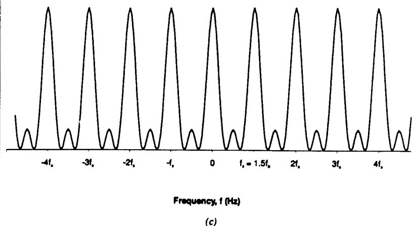
2.(a) A hypothetical FT, X_1(f) , for discussion purposes. Note that X_1(f) is generally a complex function of f , which can therefore only be correctly drawn in three dimensions. However, since x_1(t) is real and even, the FT X_1(f) happens to be real and even in this case. (b) The periodic FT Y(f) when f_s > 2f_b . (c) The periodic FT Y(f) when f_s \leq 2f_b .
