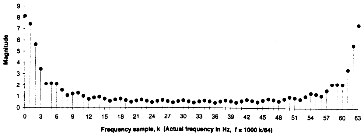
11. Magnitude spectrum of the 64-point DFT of the sequence x_3(nT_s) .
