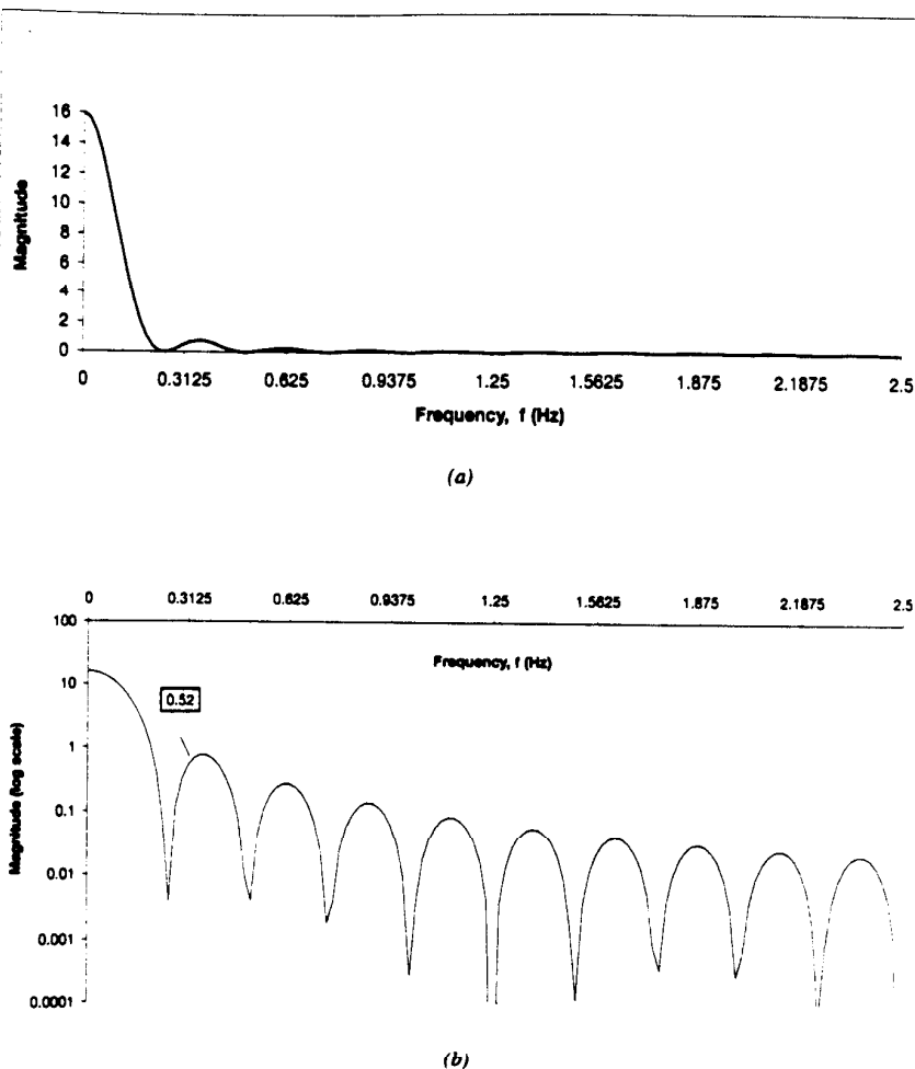
Fig. 3. "True" magnitude spectrum for the signal x_1(t) . (a) Magnitude plotted on a linear scale. (b) Log scale.
