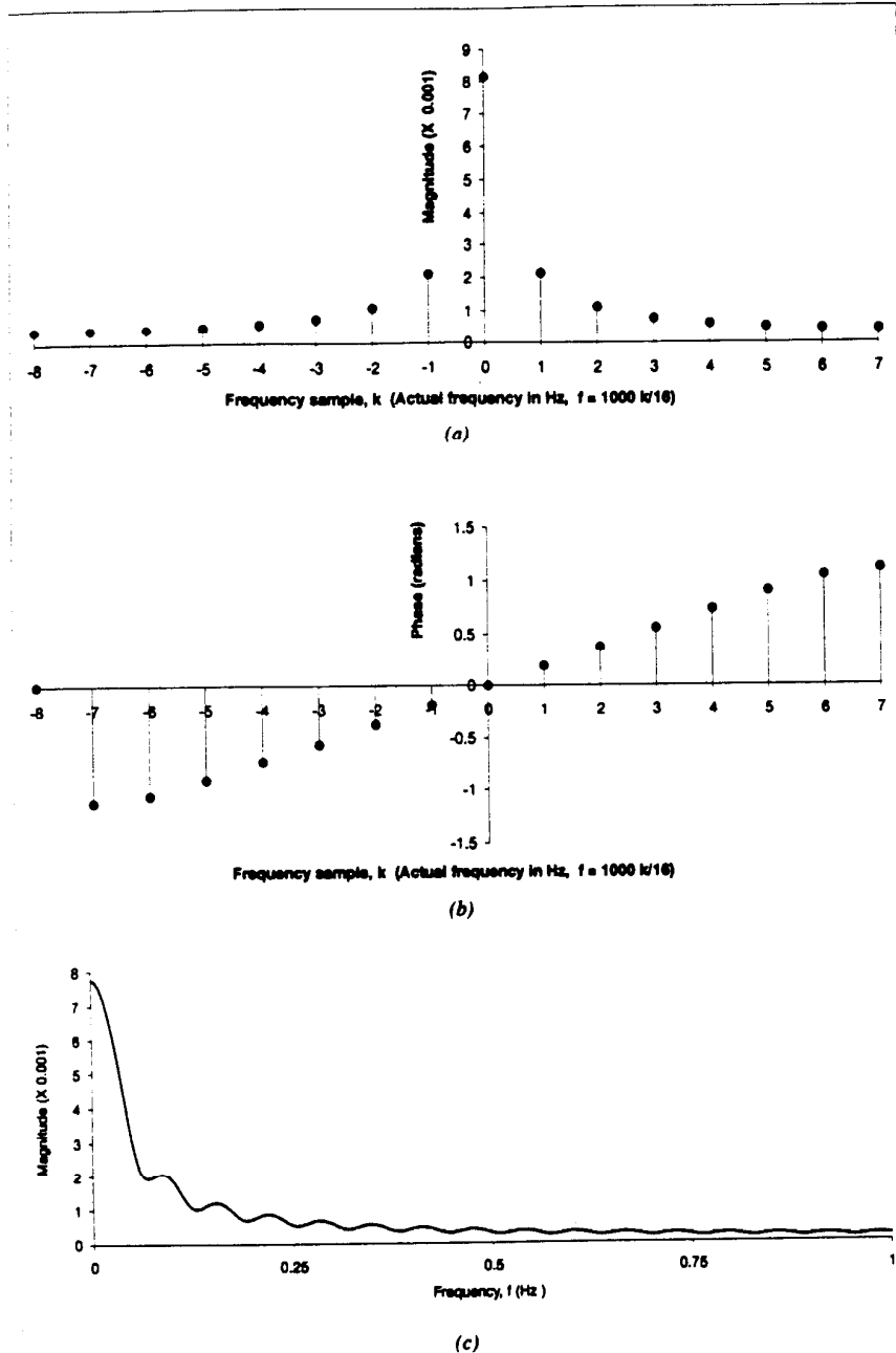
9. Samples of the (a) magnitude, and (b) phase, spectra of the discrete-time signal x_3(nT_s) of Fig. 6 obtained using Eq. 39. (c) Magnitude spectrum of the continuous-time signal x_3(t) of Eq. 21.
