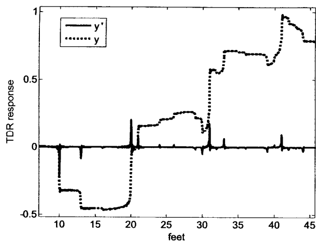
Fig. 9. Impulse response of the wire network in Fig. 3 filtered as equation (24) and its integral.
