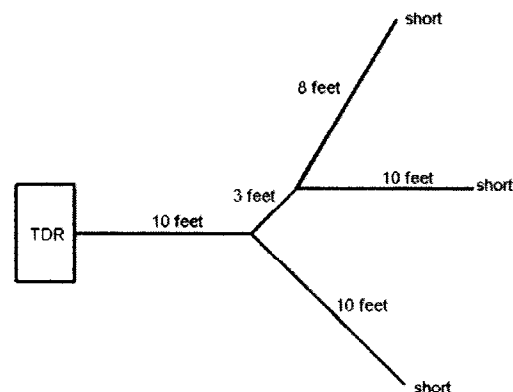
Fig. 3. Branched network to be simulated and measured with TDR. The cables are 50 ohm RG58 coaxial cable.
