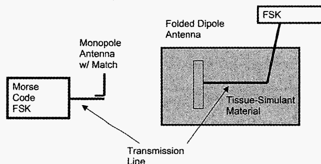
Figure 1. A block diagram of the FSK communication system for medical implants.
