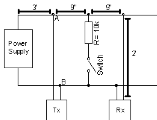
Figure 3. The basic setup for testing the effect of staged intermittent faults in parallel to the power supply on the messages transmitted using PLC.
