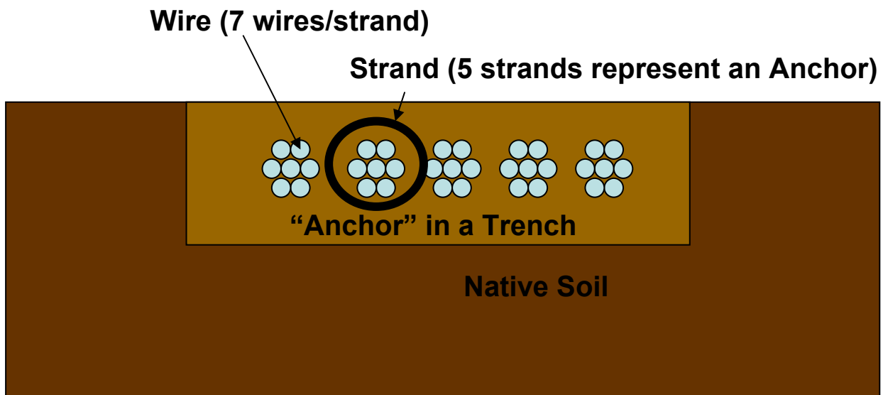
Figure 3 Cross Section of Simulated Anchor for this Test. Another identical anchor in another trench a few feet away was used as the 'ground' reference.
