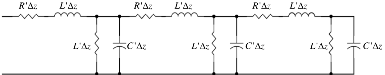
Figure 4 Lumped element (RLGC) model of a transmission line
