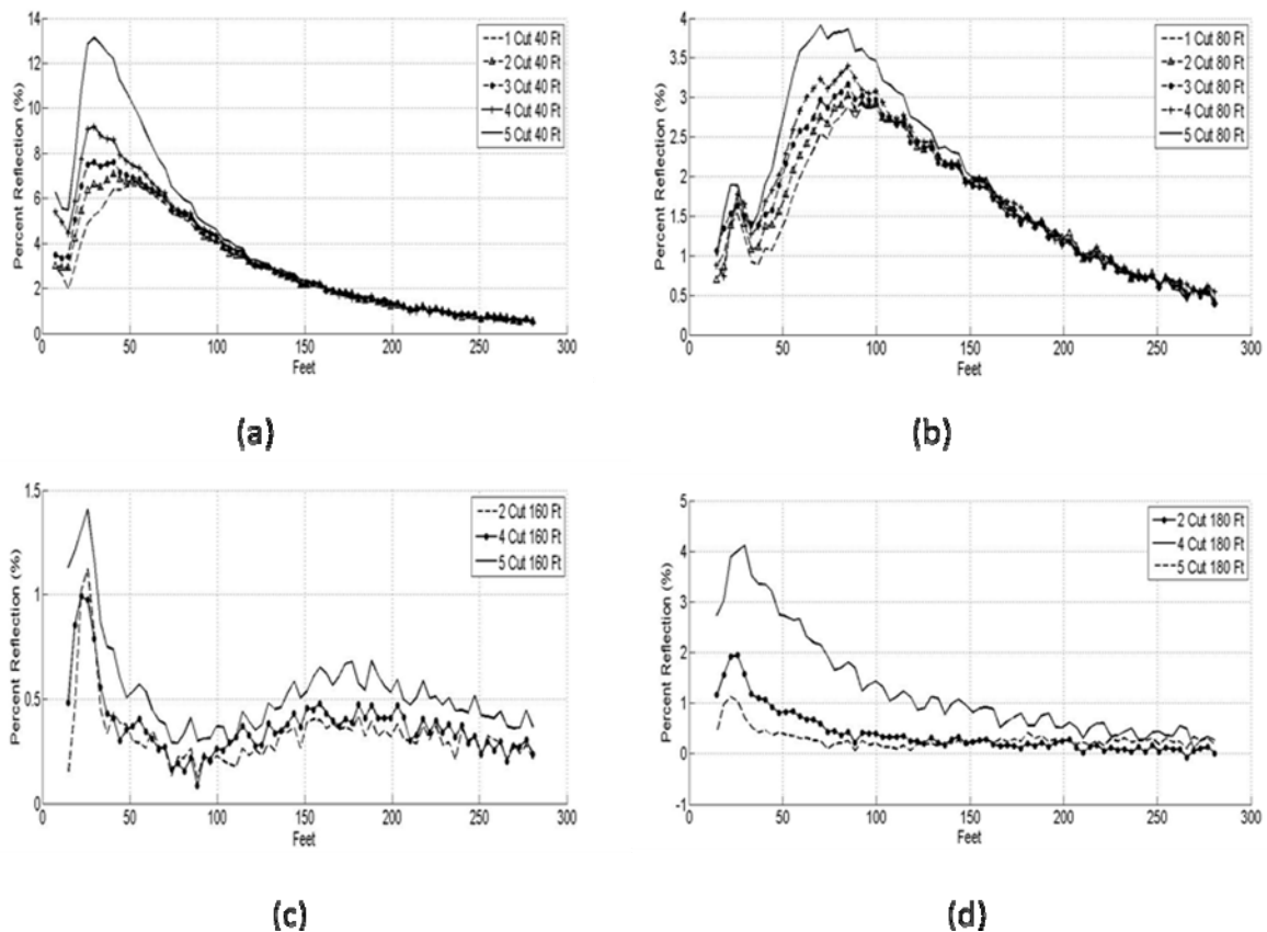
Figure 18 Partially Damaged Anchors showing effect of cutting 1,2,3,4 or 5 strands. (a) Cuts at 40', (b) cuts at 80', (c) cuts at 160', (d) cuts at 180'. All data is compared to a baseline at 200'. All anchors are in trenches 7' apart. For cuts up to 160' it appears that partial damage to the anchor can be identified.
