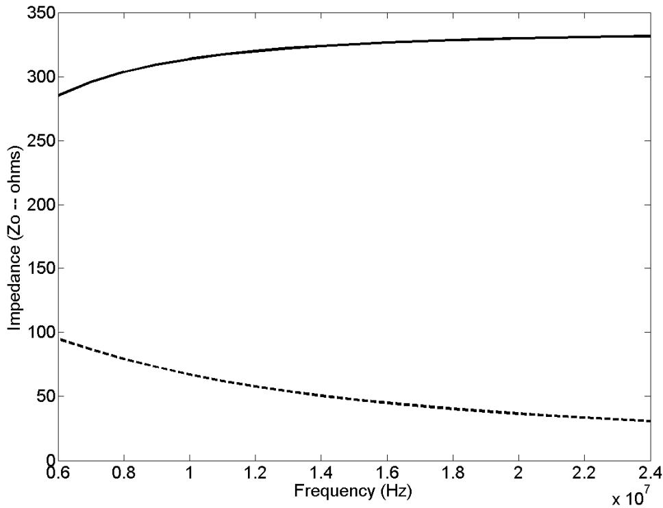
Figure 8 Impedance ( Z_o ) of steel anchors as a function of frequency. The electrical properties of concrete / dirt are \epsilon_r=4 and \sigma = 1 mS/m. The anchor is a 5/8" diameter steel anchor with a trench spacing of 7'. The real part of the impedance is shown in the solid lines, and the imaginary part is shown in the dashed lines.
