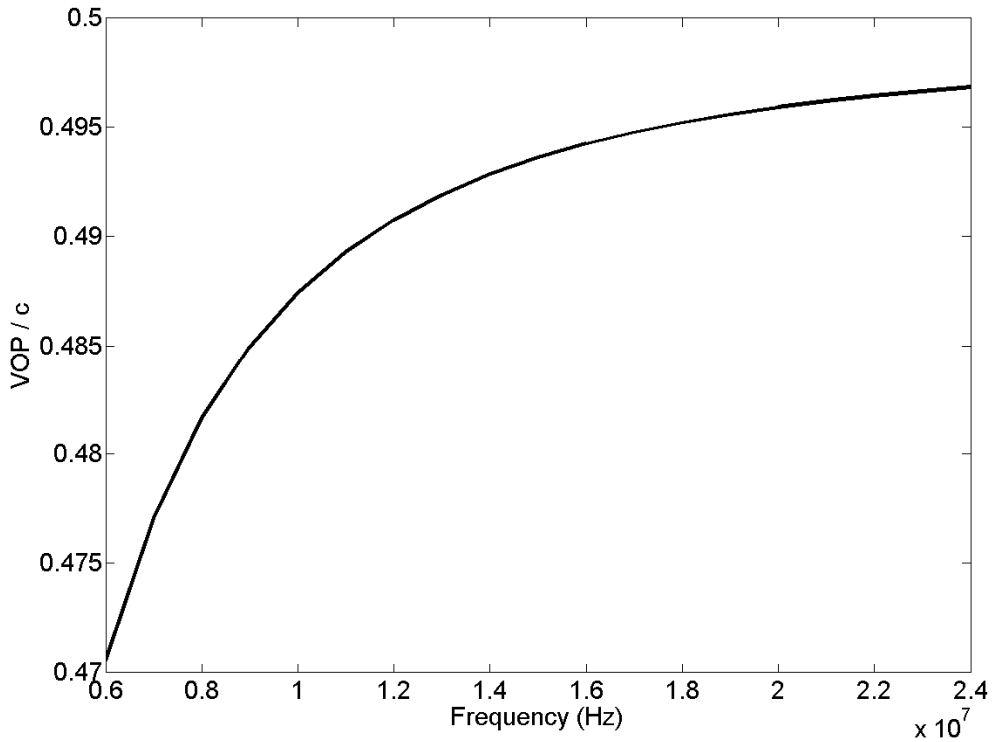
Figure 9 Velocity of propagation (vop) of steel anchors as a function of frequency. The electrical properties of concrete / dirt are \epsilon_r=4 and \sigma = 1 mS/m. The anchor is a 5/8" diameter steel anchor with a trench spacing of 7'.
