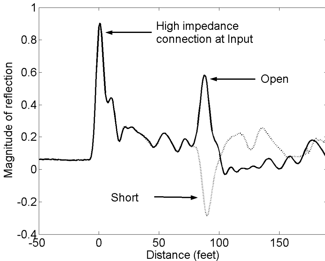
Figure 1 STDR responses for an 80 foot wire (paired single 22 gauge wires bundled with other wires) that is short or open circuited on the end.
