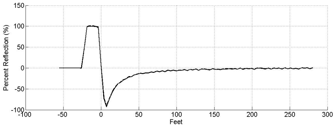
Figure 16 Example Baseline collected from two 200' wires 7 feet apart.
