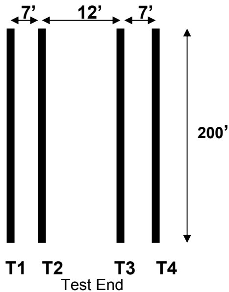
Figure 12 Four parallel trenches were used simulate anchors in concrete.
