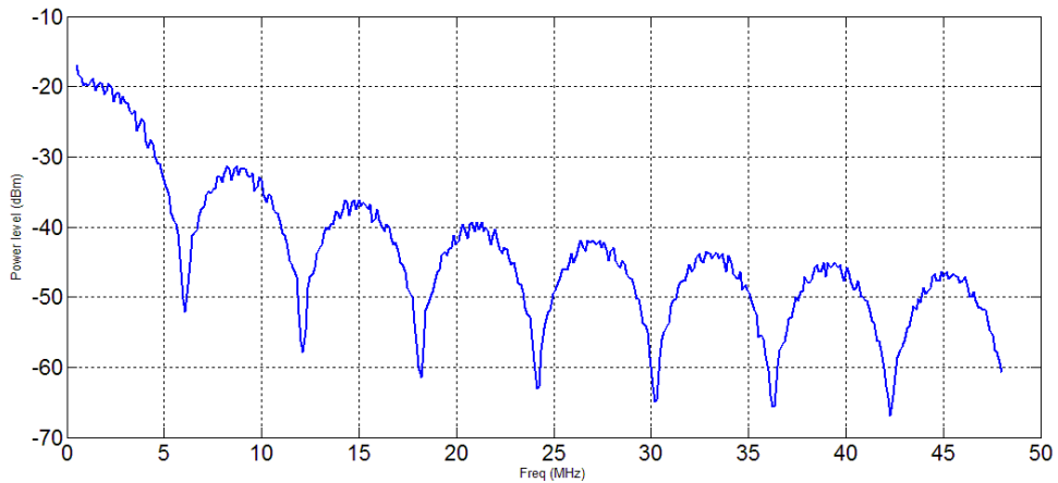
Figure 11 Frequency spectrum of the 6 MHz STDR signals.
