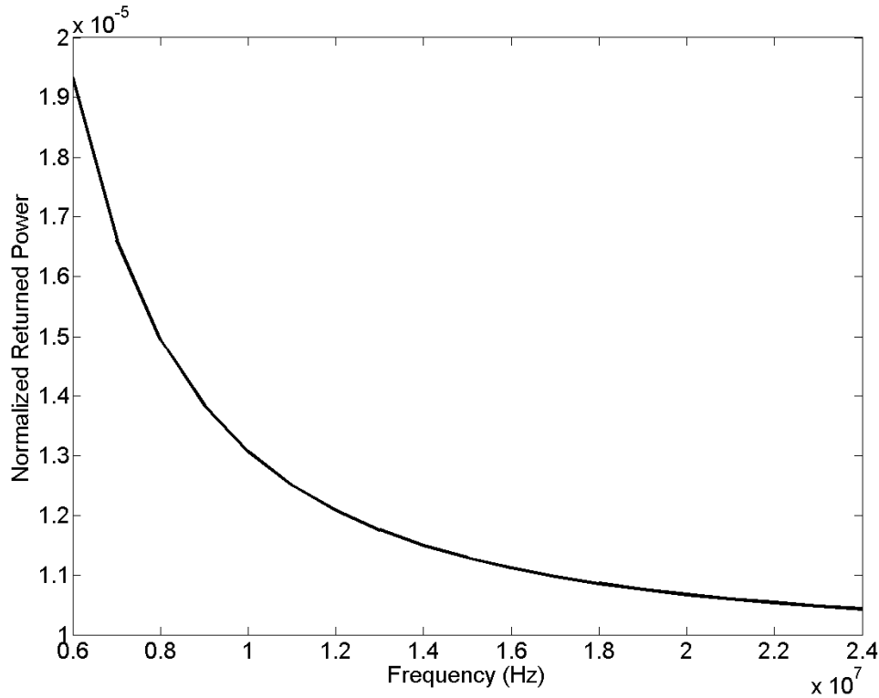
Figure 10 Attenuation of steel anchors as a function of frequency. The electrical properties of concrete / dirt are \epsilon_r=4 and \sigma = 1 mS/m. The anchor is a 5/8" diameter steel anchor with a trench spacing of 7'.
