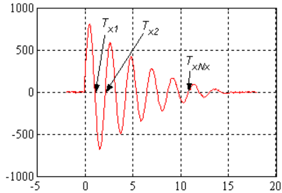
Figure 15. Measured current zero crossings.
