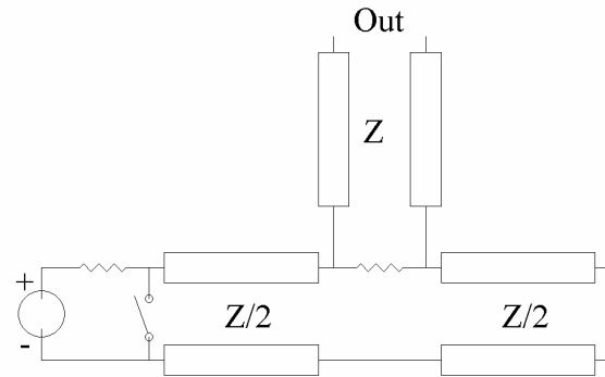
Figure 2. Blumlein pulser
