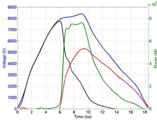
Figure 26. Input (blue), transmitted (black), and reflected voltage (red) pulses. Also shown is the power pulse into the arc (green).
