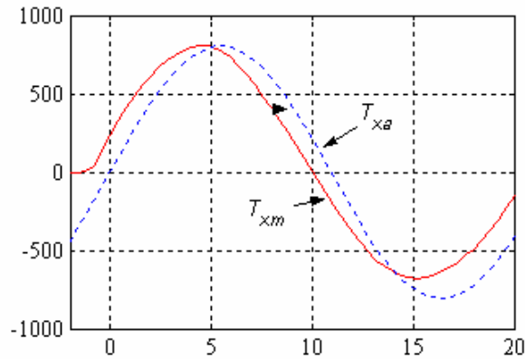
Figure 16. Measured current phase shift correction.
